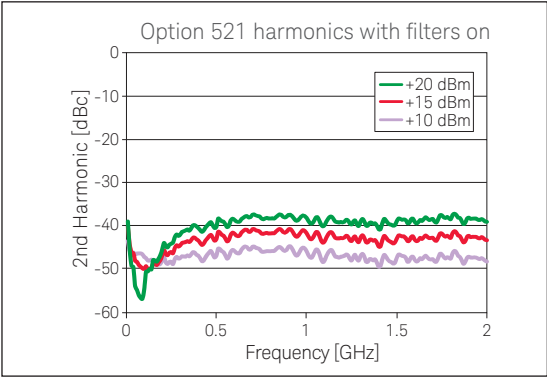
Harmonics (measured)
