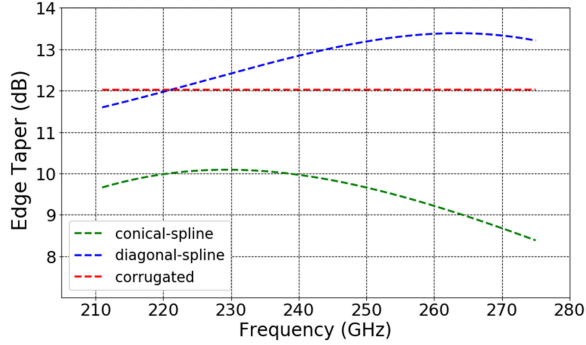
Fig. 6. Edge taper versus frequency when the Band-6 optical system is fed by different horns antennas.
