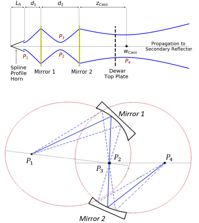
Fig. 5. (Top) Optical train description of the ALMA Band-6 optics, which consists of two elliptical mirrors (represented by yellow lines), and the spline-profile horn. The final beam waist and its position respect to mirror 2 are given by w_{cass} and z_{cass} , respectively. (Bottom) Mirror layout of ALMA Band-6 cold optical system. The points P_1 and P_2 represent the position of focal points for the mirror 1; P_3 and P_4 have the same relation with the mirror 2. The chief ray is shown by solid blue line.
