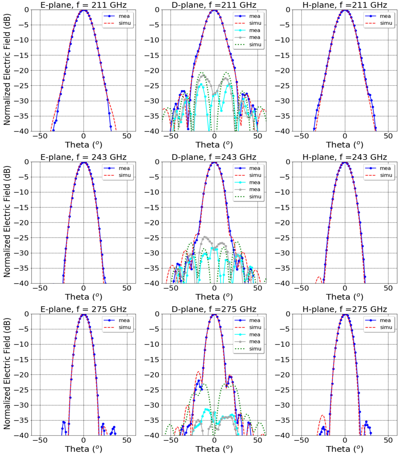
Fig. 12. Comparison between experimental results (dotted lines) and simulations (dashed lines) for the far-field radiation pattern. Copolar comparison was made taking the cross section along the E and H planes (left and right column respectively), whereas cross-polar comparison (middle column) was made taking two cross sections at 45^\circ (cyan) and 135^\circ (gray), as shown in Fig. 11, using the same colors to facilitate the visualization.
