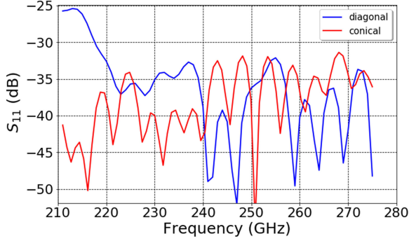
Fig. 4. Simulated return loss for diagonal-spline and conical-spline horns. Both designs show return loss levels below -25 dB for the entire frequency range.
