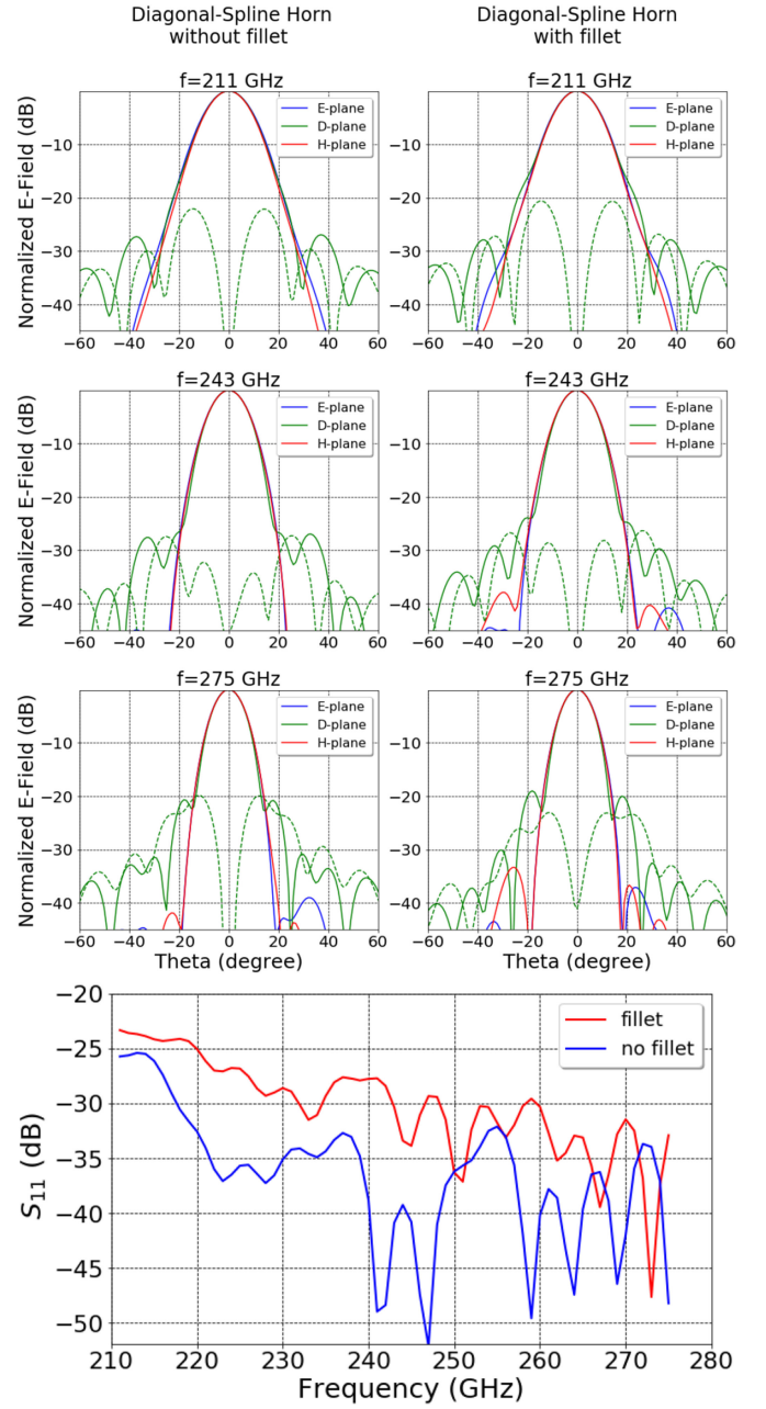
Fig. 7. (Top) Simulated far-field radiation pattern for the diagonal-spline horn with and without fillet. When the fillet is included the main difference is on cross polar (dashed line), which suffers a small degradation at 211 and 243 GHz but improves at 275 GHz. (Bottom) Return loss comparison. Small differences are visible, but performance is till < -23 dB over the entire frequency range.
